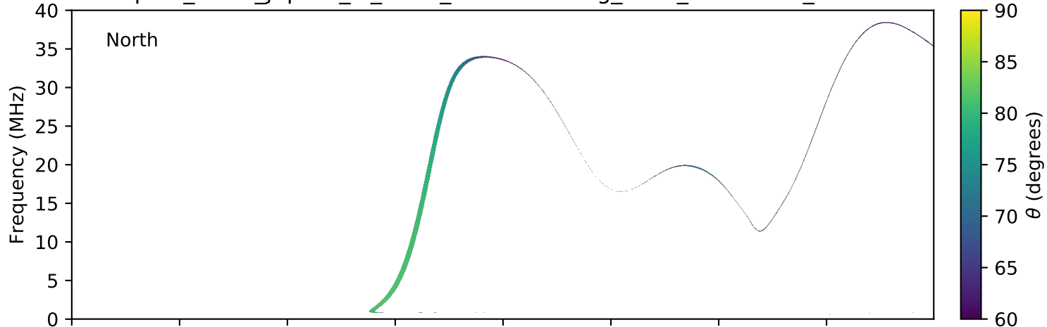
expres_earth_jupiter_io_isaac_lossc-wid1deg_5kev_20160602_v01.cdf
