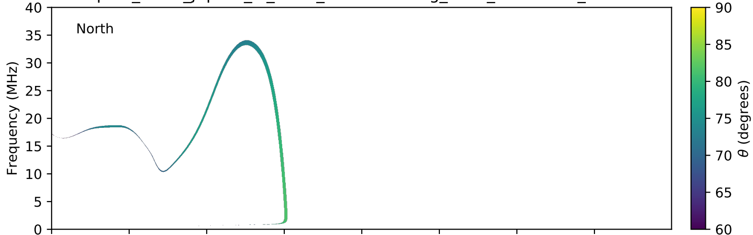
expres_earth_jupiter_io_isaac_lossc-wid1deg_5kev_20160601_v01.cdf
