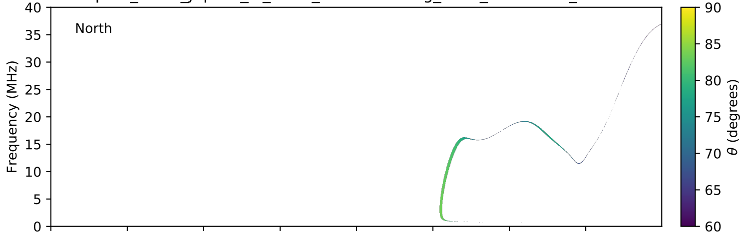
expres_earth_jupiter_io_isaac_lossc-wid1deg_3kev_20160630_v01.cdf
