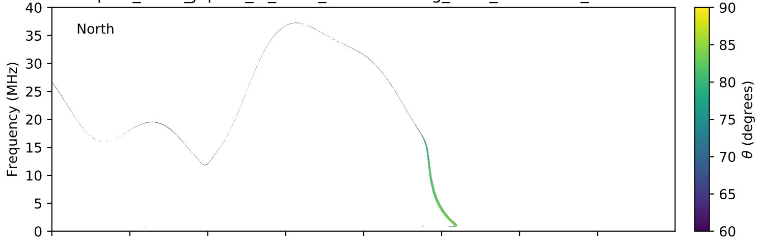
expres_earth_jupiter_io_isaac_lossc-wid1deg_3kev_20160629_v01.cdf
