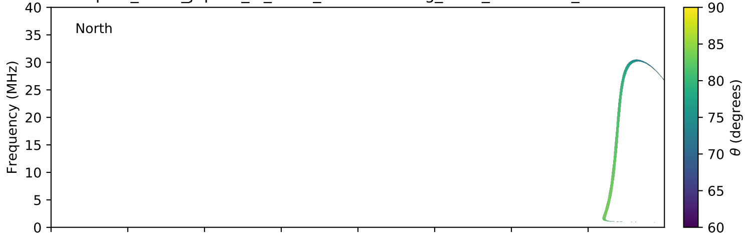
expres_earth_jupiter_io_isaac_lossc-wid1deg_3kev_20160628_v01.cdf
