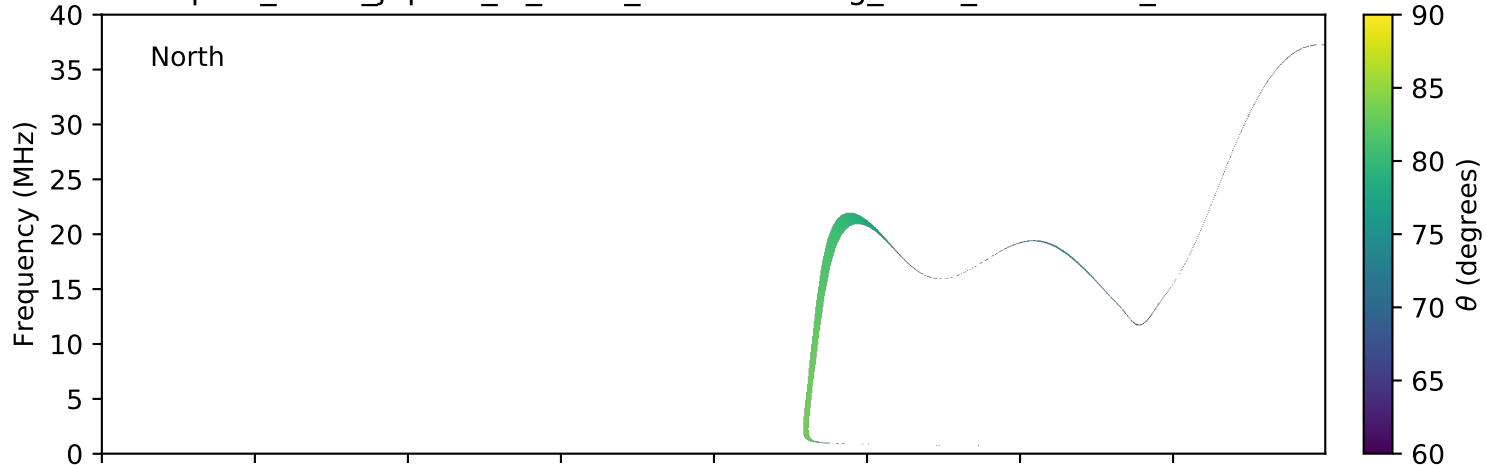
expres_earth_jupiter_io_isaac_lossc-wid1deg_3kev_20160623_v01.cdf
