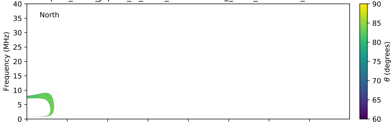
expres_earth_jupiter_io_isaac_lossc-wid1deg_3kev_20160619_v01.cdf
