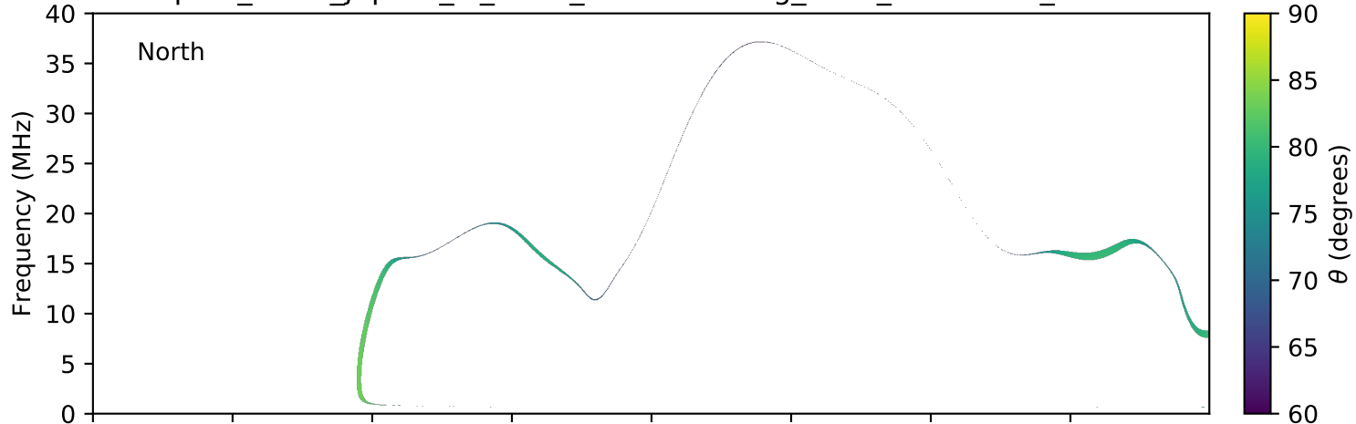
expres_earth_jupiter_io_isaac_lossc-wid1deg_3kev_20160618_v01.cdf
