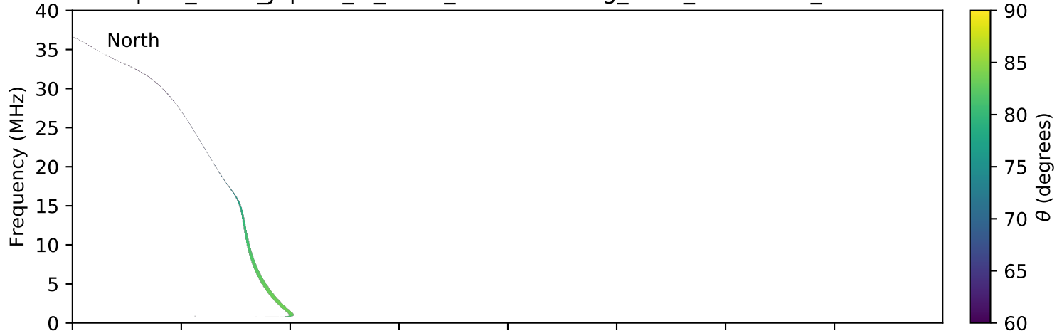
expres_earth_jupiter_io_isaac_lossc-wid1deg_3kev_20160617_v01.cdf
