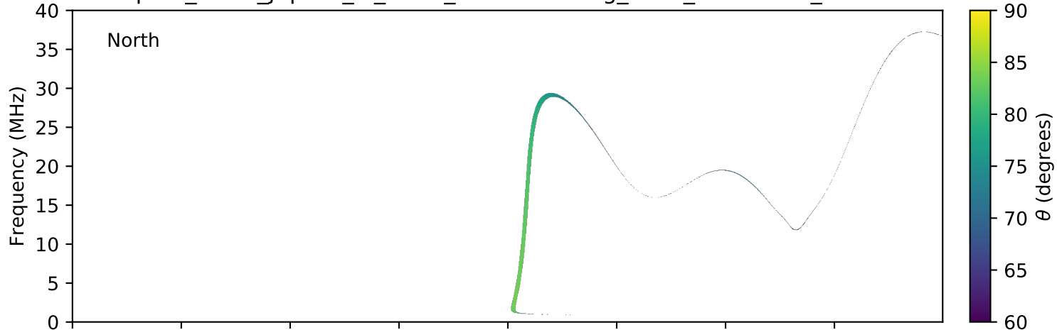
expres_earth_jupiter_io_isaac_lossc-wid1deg_3kev_20160616_v01.cdf
