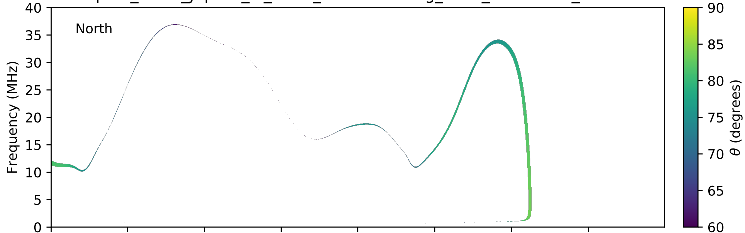
expres_earth_jupiter_io_isaac_lossc-wid1deg_3kev_20160613_v01.cdf
