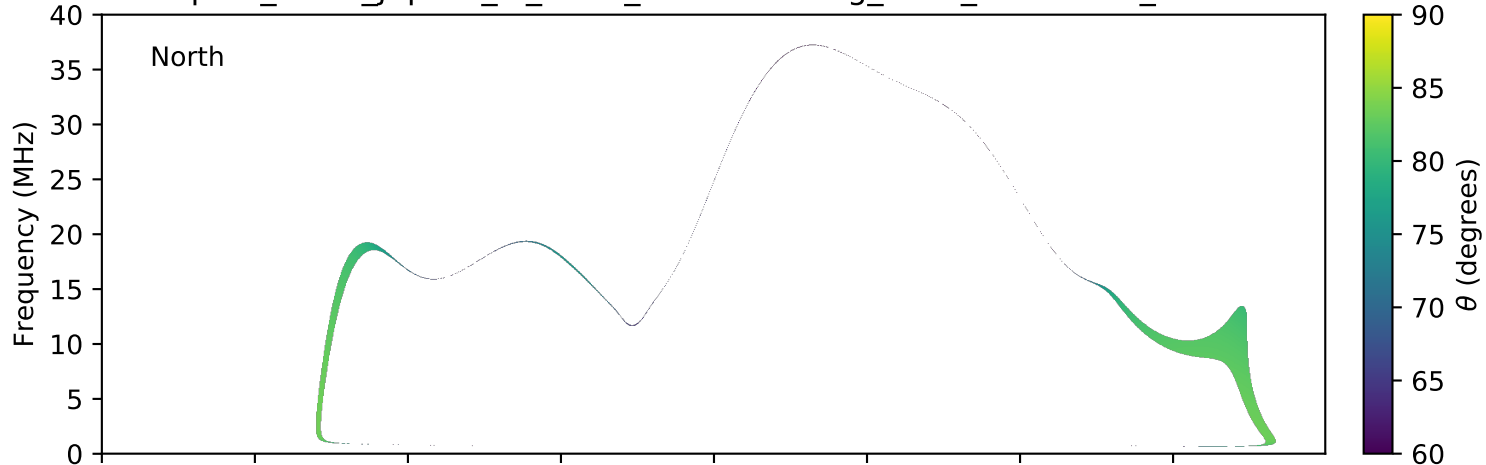
expres_earth_jupiter_io_isaac_lossc-wid1deg_3kev_20160611_v01.cdf
