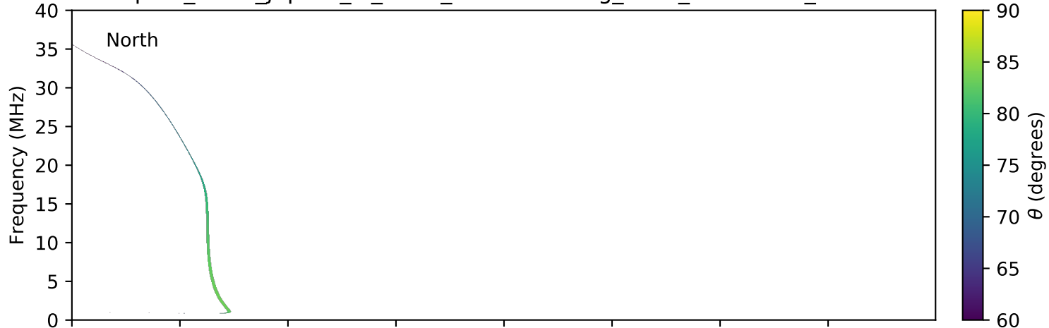
expres_earth_jupiter_io_isaac_lossc-wid1deg_3kev_20160610_v01.cdf
