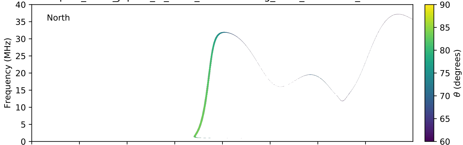
expres_earth_jupiter_io_isaac_lossc-wid1deg_3kev_20160609_v01.cdf
