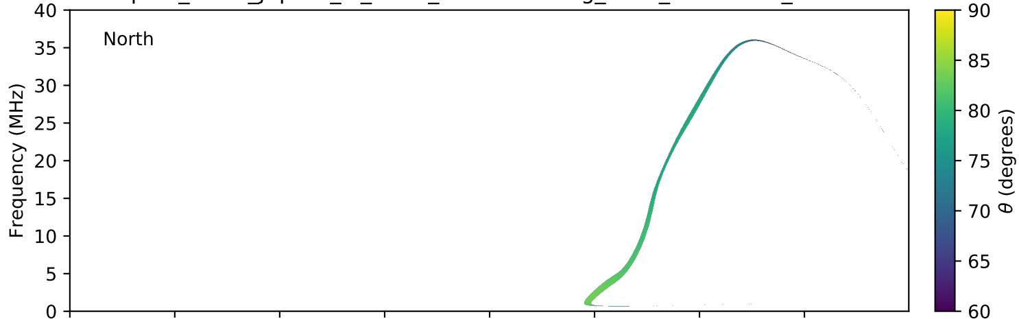
expres_earth_jupiter_io_isaac_lossc-wid1deg_3kev_20160607_v01.cdf
