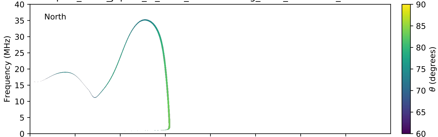
expres_earth_jupiter_io_isaac_lossc-wid1deg_3kev_20160601_v01.cdf
