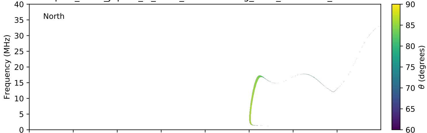
expres_earth_jupiter_io_isaac_lossc-wid1deg_1kev_20160630_v01.cdf
