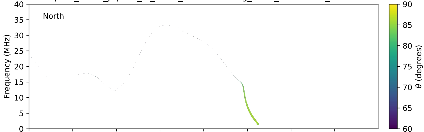
expres_earth_jupiter_io_isaac_lossc-wid1deg_1kev_20160629_v01.cdf
