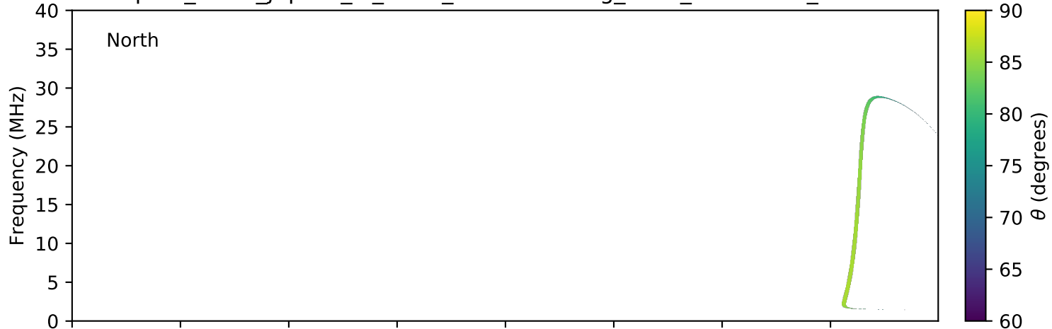
expres_earth_jupiter_io_isaac_lossc-wid1deg_1kev_20160628_v01.cdf
