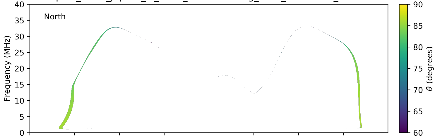
expres_earth_jupiter_io_isaac_lossc-wid1deg_1kev_20160627_v01.cdf
