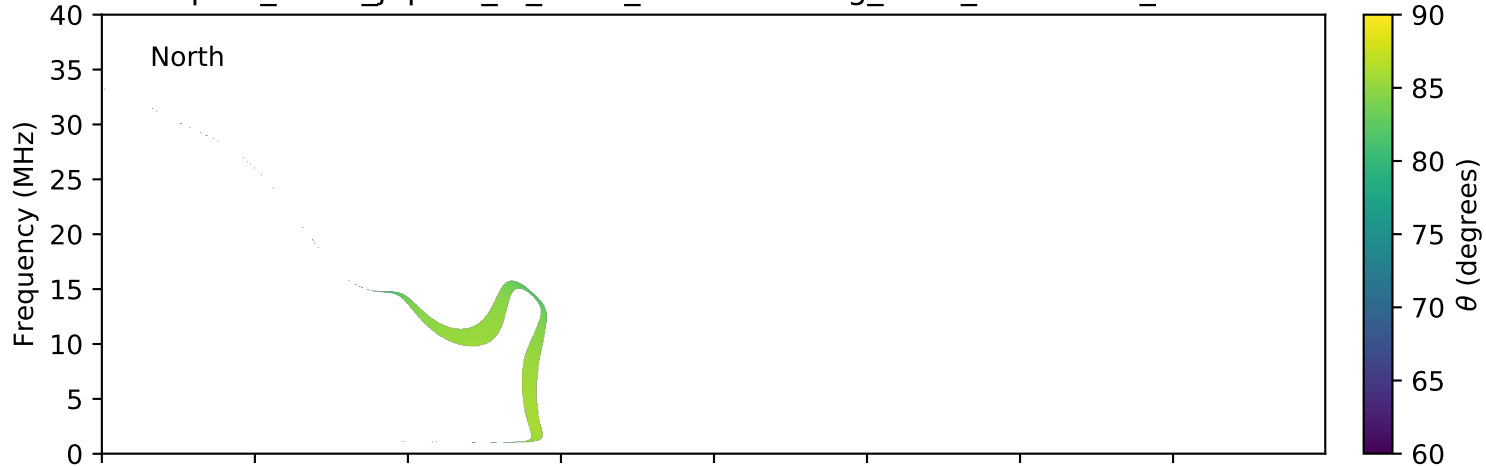
expres_earth_jupiter_io_isaac_lossc-wid1deg_1kev_20160624_v01.cdf
