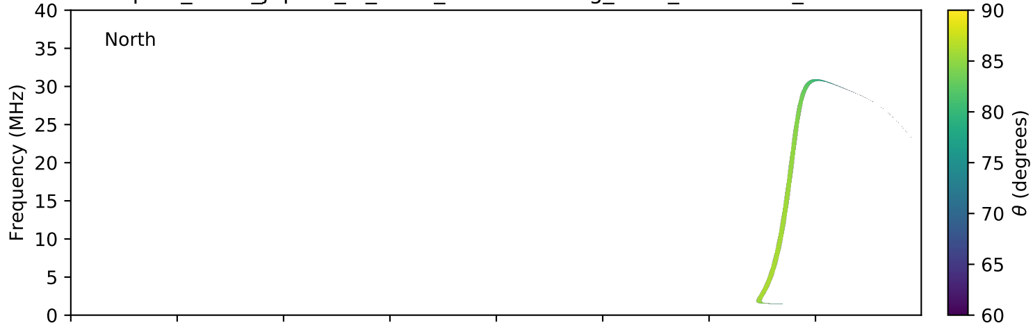
expres_earth_jupiter_io_isaac_lossc-wid1deg_1kev_20160621_v01.cdf
