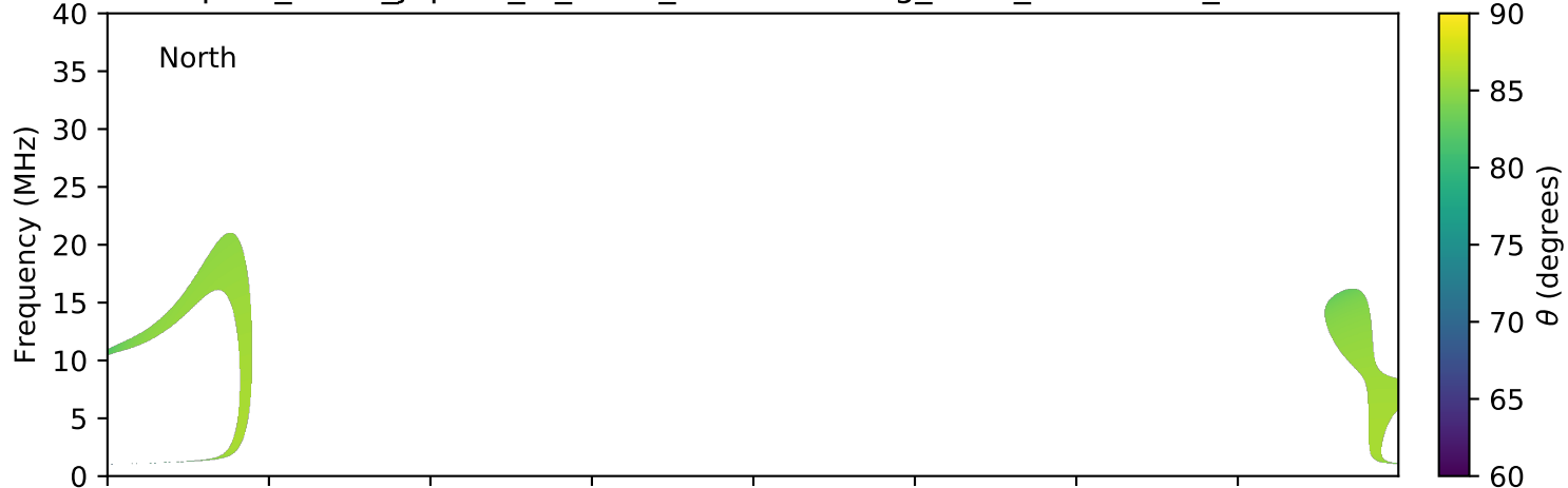
expres_earth_jupiter_io_isaac_lossc-wid1deg_1kev_20160619_v01.cdf
