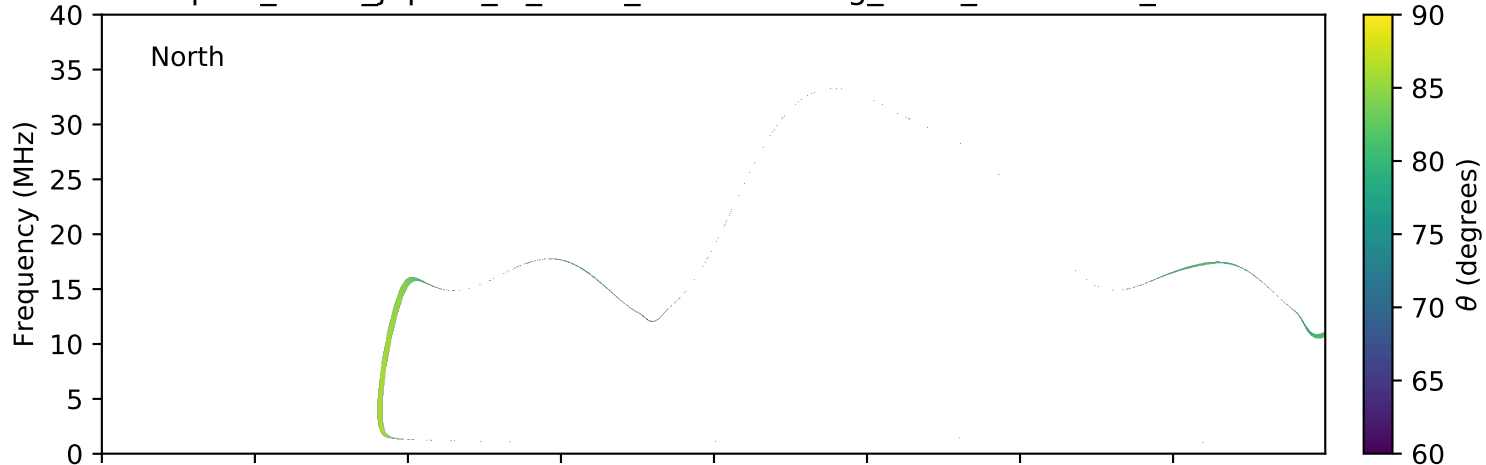
expres_earth_jupiter_io_isaac_lossc-wid1deg_1kev_20160618_v01.cdf
