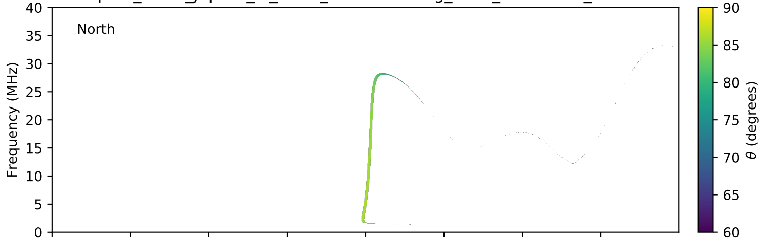
expres_earth_jupiter_io_isaac_lossc-wid1deg_1kev_20160616_v01.cdf
