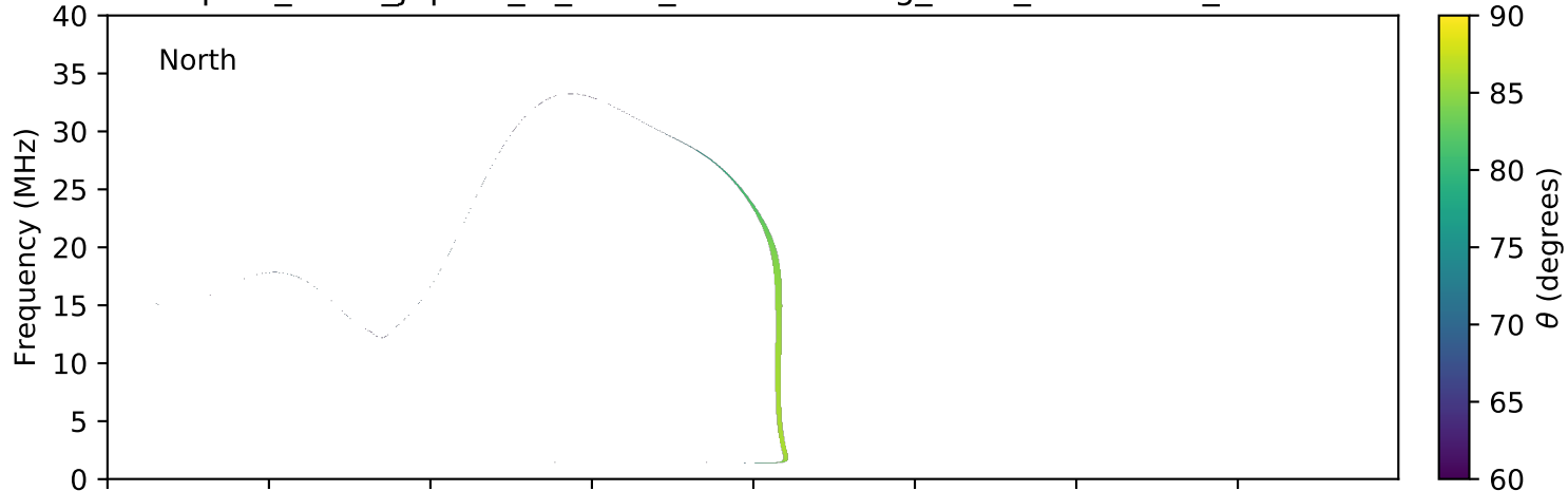
expres_earth_jupiter_io_isaac_lossc-wid1deg_1kev_20160615_v01.cdf
