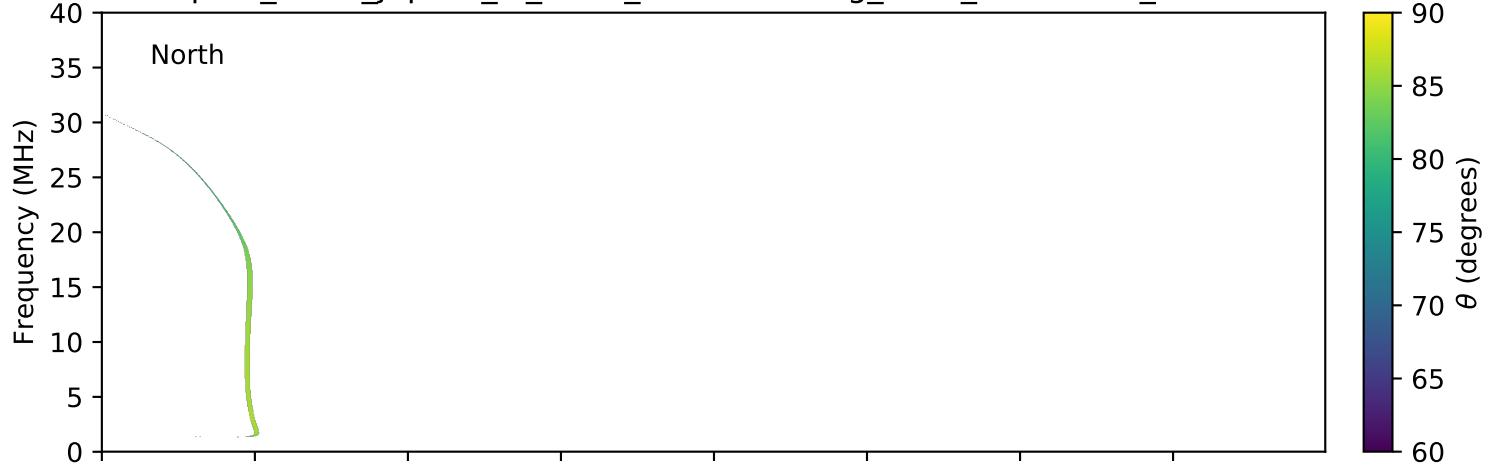
expres_earth_jupiter_io_isaac_lossc-wid1deg_1kev_20160603_v01.cdf
