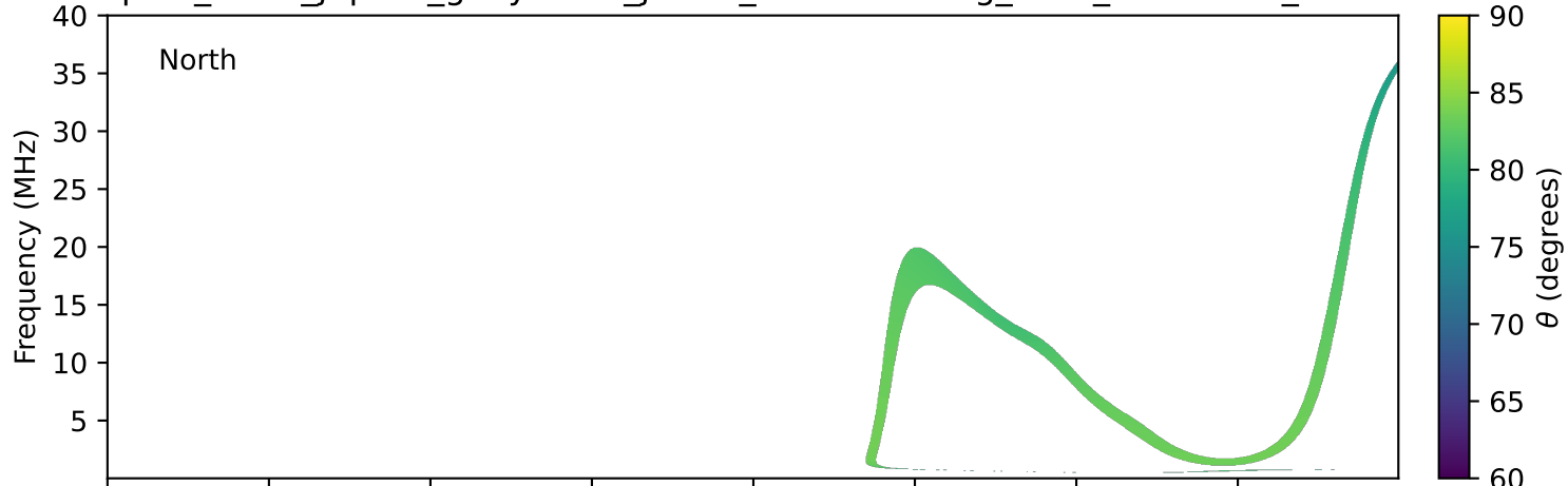
expres_earth_jupiter_ganymede_jrm33_lossc-wid1deg_3kev_20160630_v11.cdf
