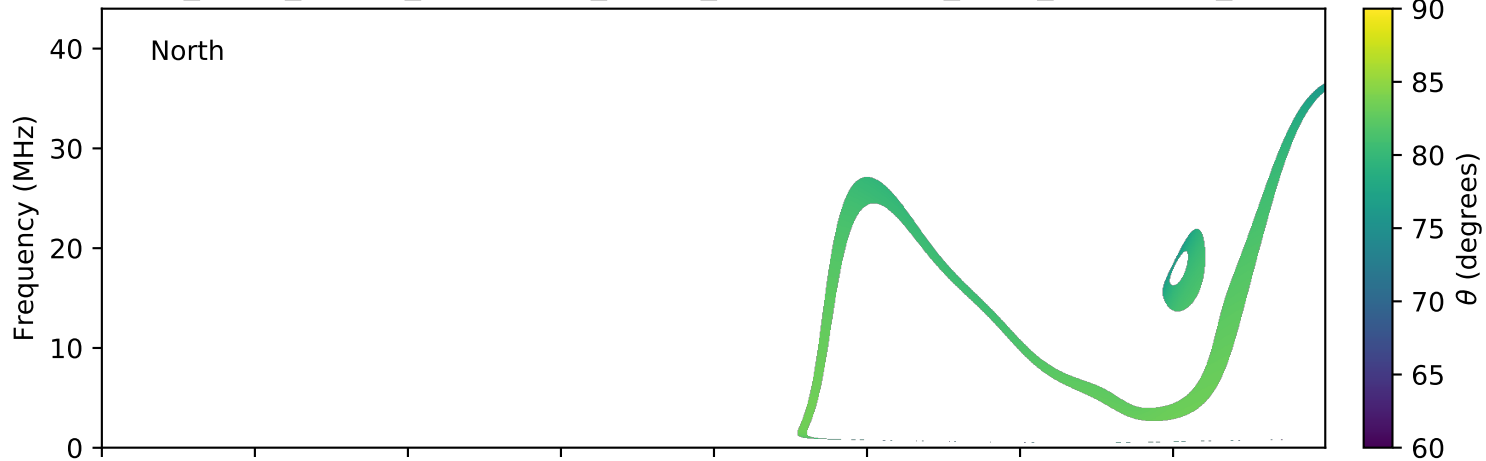
expres_earth_jupiter_ganymede_jrm09_lossc-wid1deg_3kev_20160630_v01.cdf
