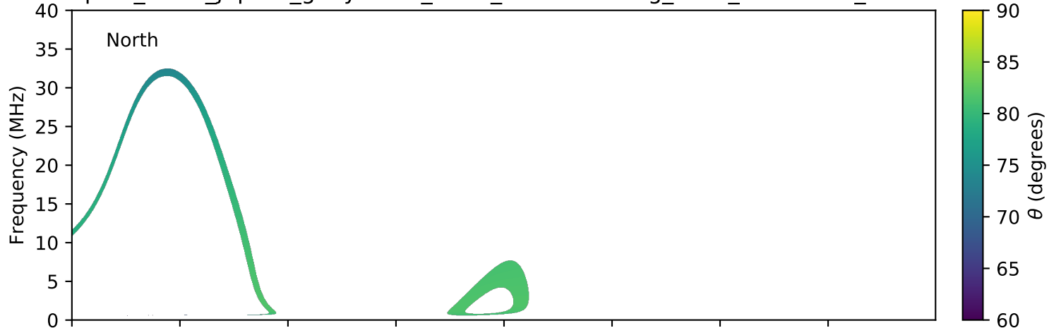
expres_earth_jupiter_ganymede_isaac_lossc-wid1deg_5kev_20160619_v01.cdf
