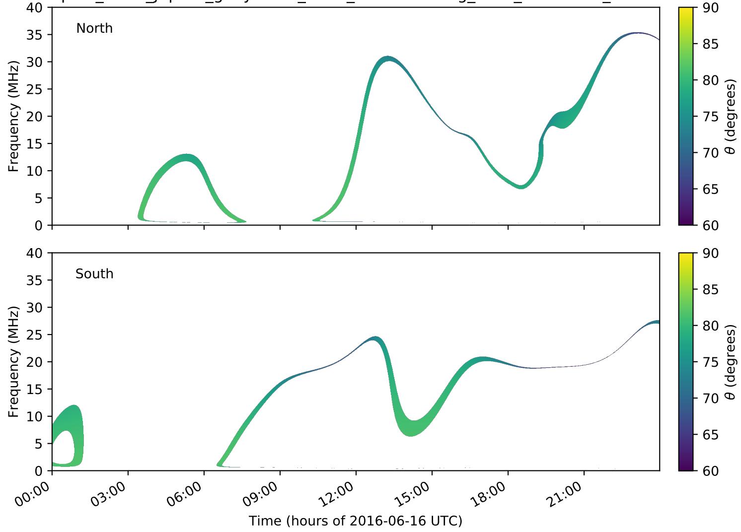
expres_earth_jupiter_ganymede_isaac_lossc-wid1deg_5kev_20160616_v01.cdf
