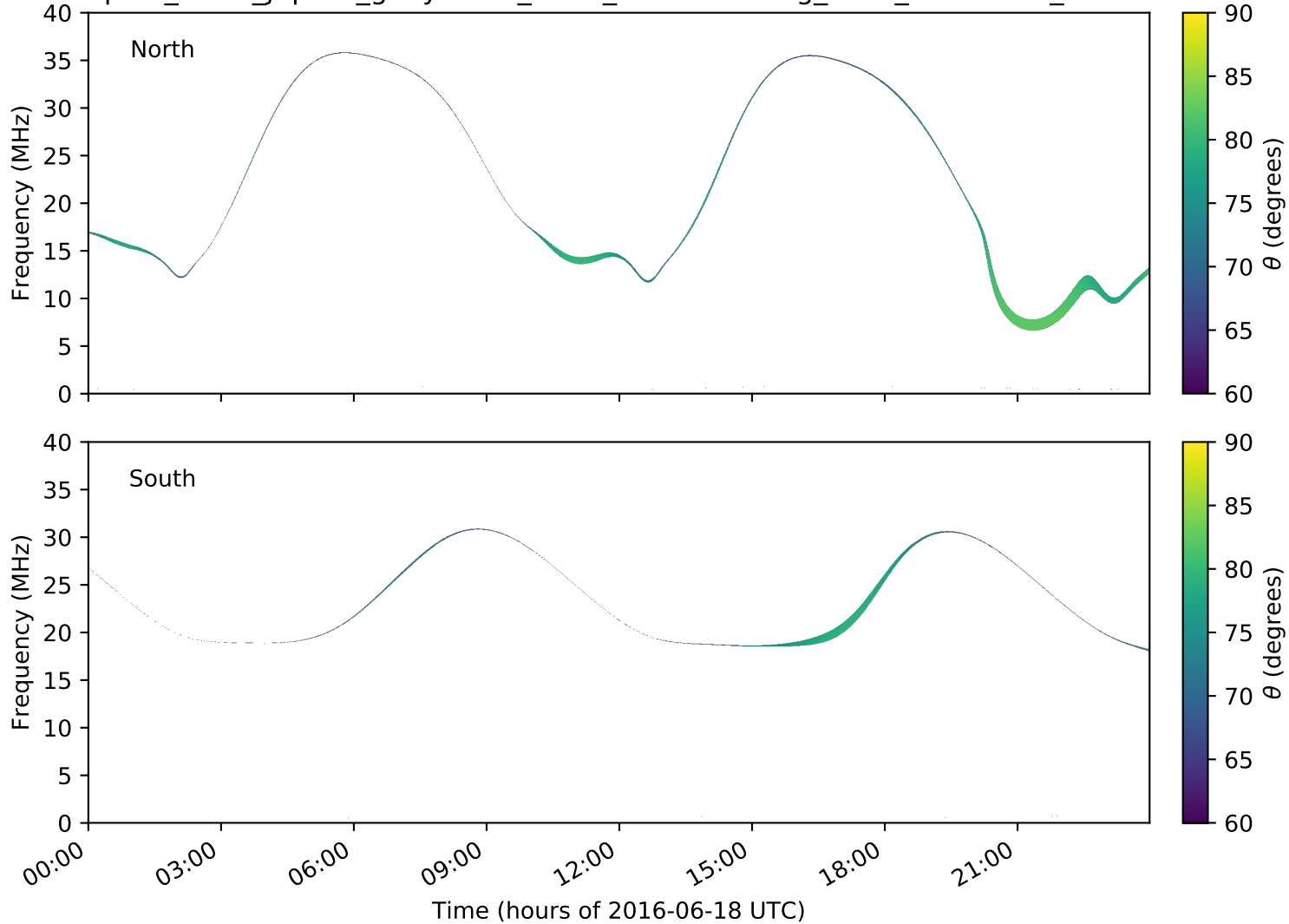
expres_earth_jupiter_ganymede_isaac_lossc-wid1deg_3kev_20160618_v01.cdf
