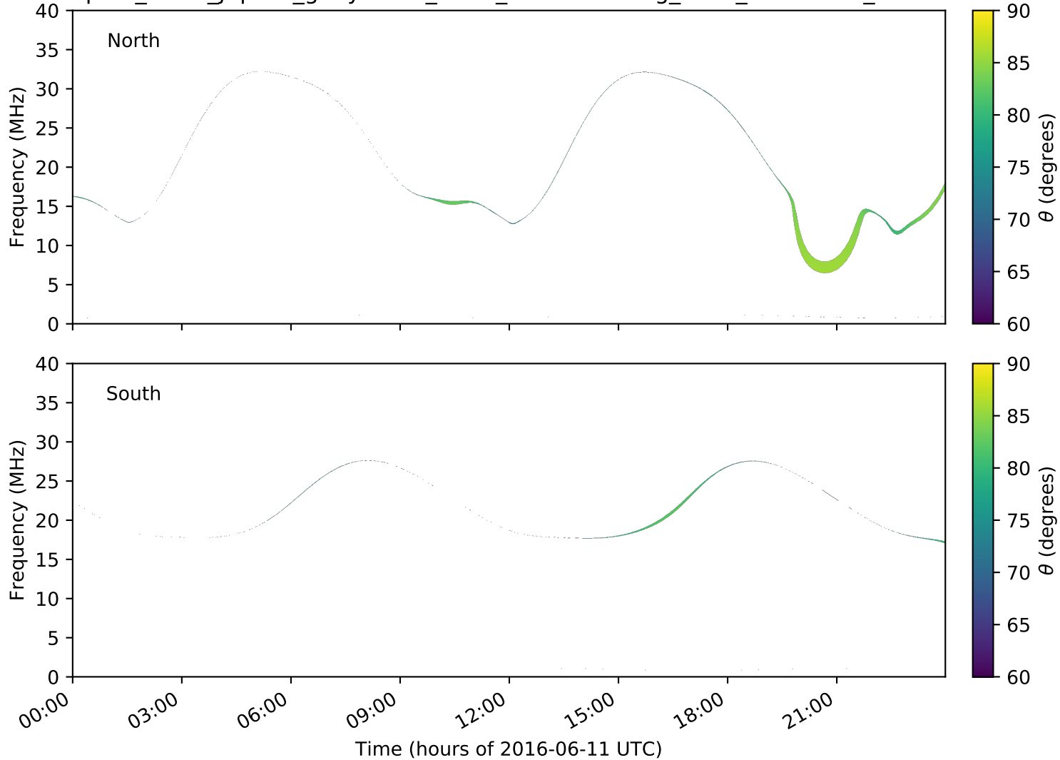
expres_earth_jupiter_ganymede_isaac_lossc-wid1deg_1kev_20160611_v01.cdf
