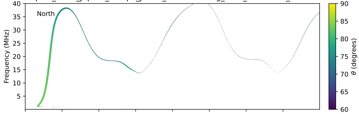
expres_earth_jupiter_europa_jrm33_lossc-wid1deg_3kev_20160604_v11.cdf
