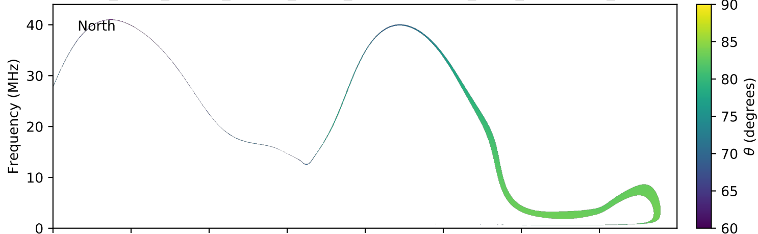
expres_earth_jupiter_europa_jrm09_lossc-wid1deg_3kev_20160626_v01.cdf
