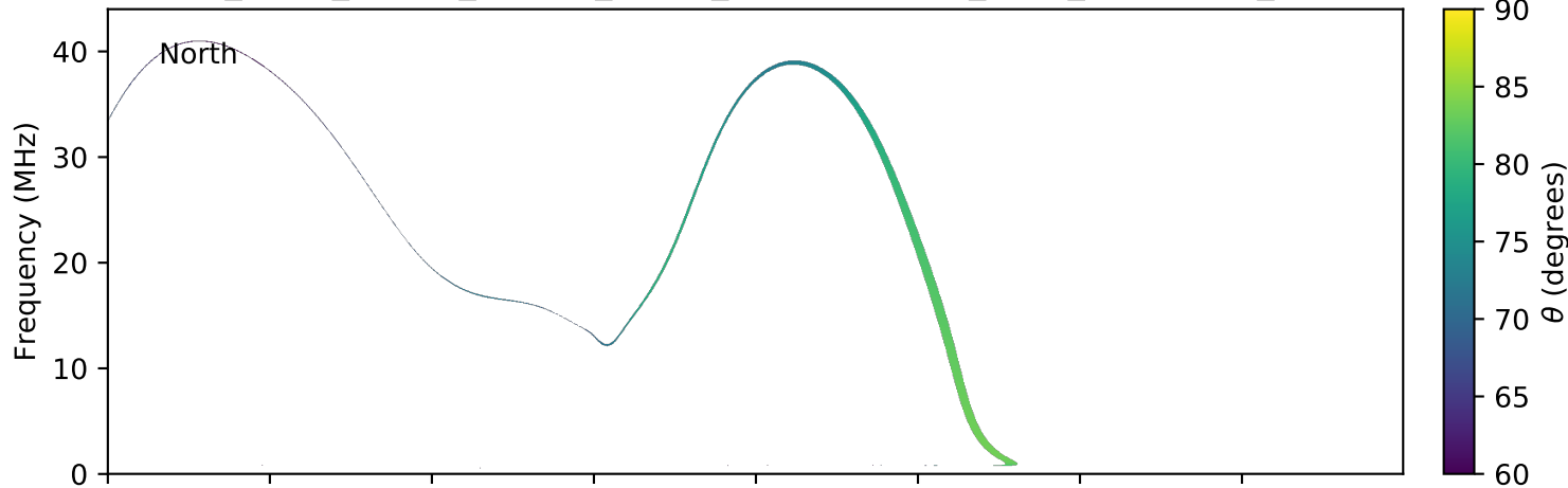
expres_earth_jupiter_europa_jrm09_lossc-wid1deg_3kev_20160619_v01.cdf
