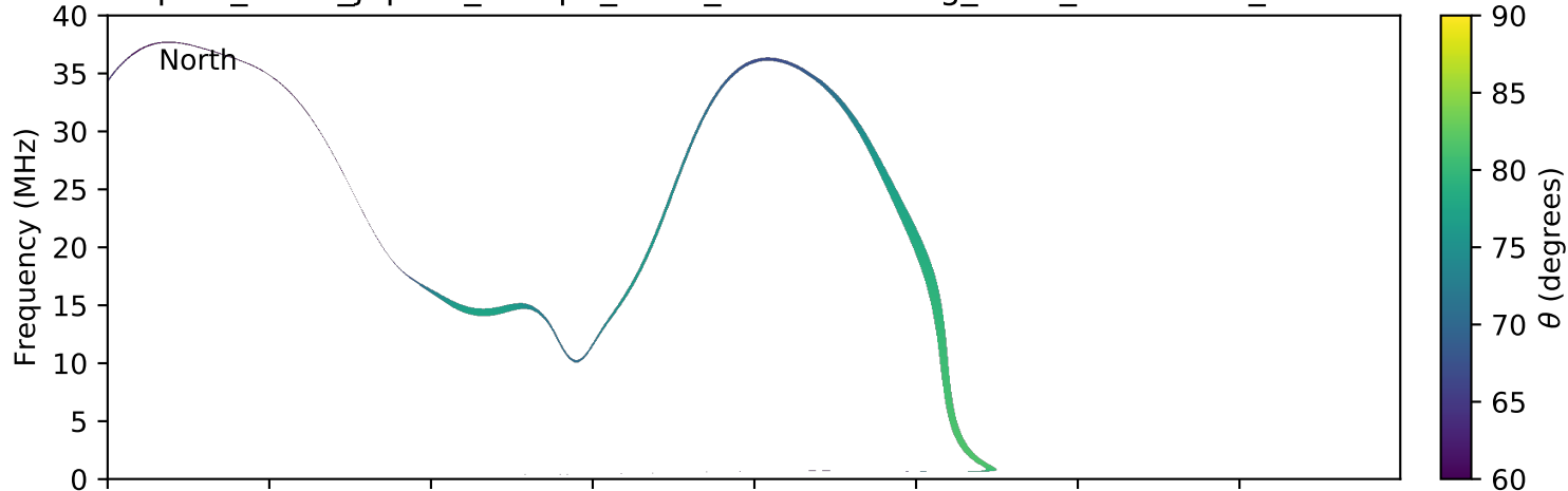
expres_earth_jupiter_europa_isaac_lossc-wid1deg_5kev_20160619_v01.cdf
