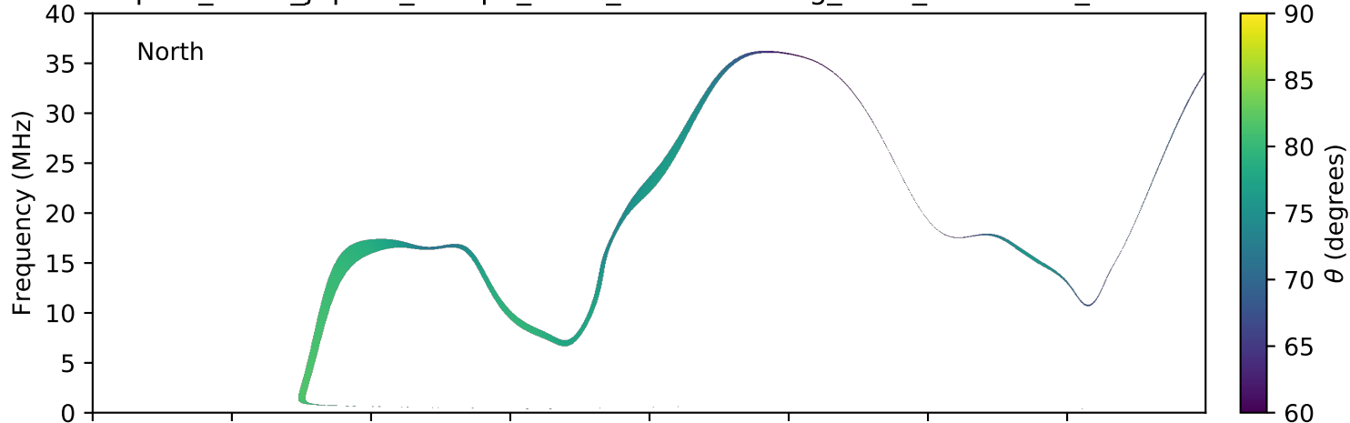
expres_earth_jupiter_europa_isaac_lossc-wid1deg_5kev_20160618_v01.cdf
