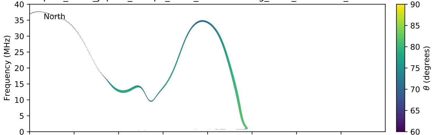
expres_earth_jupiter_europa_isaac_lossc-wid1deg_5kev_20160612_v01.cdf
