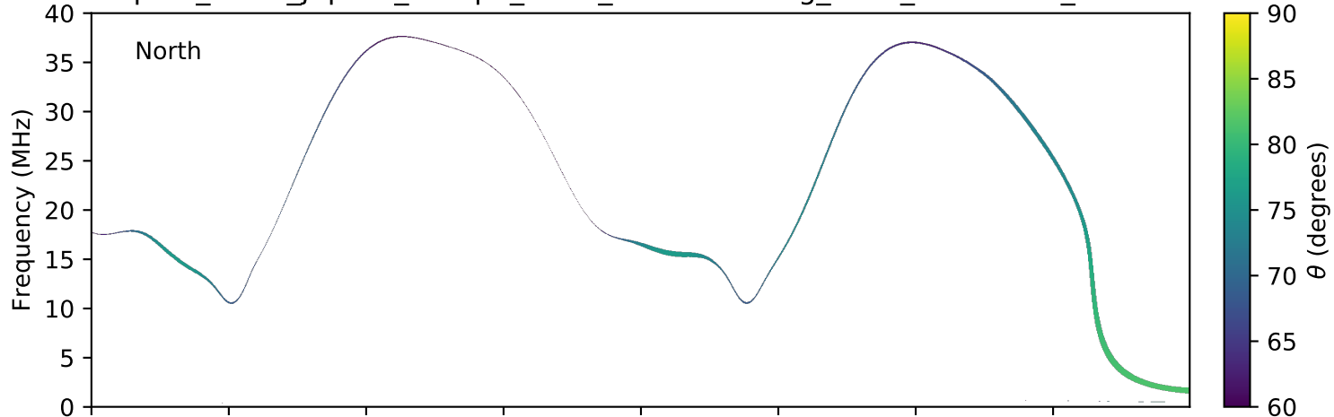
expres_earth_jupiter_europa_isaac_lossc-wid1deg_5kev_20160608_v01.cdf
