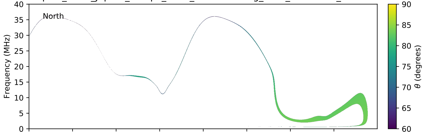
expres_earth_jupiter_europa_isaac_lossc-wid1deg_3kev_20160626_v01.cdf
