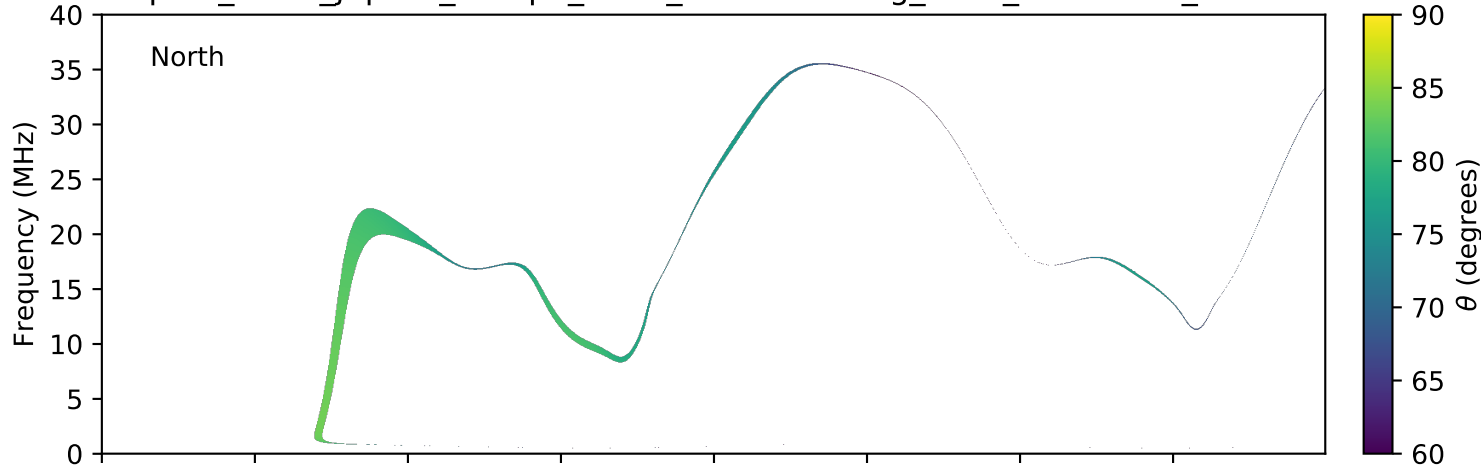
expres_earth_jupiter_europa_isaac_lossc-wid1deg_3kev_20160618_v01.cdf
