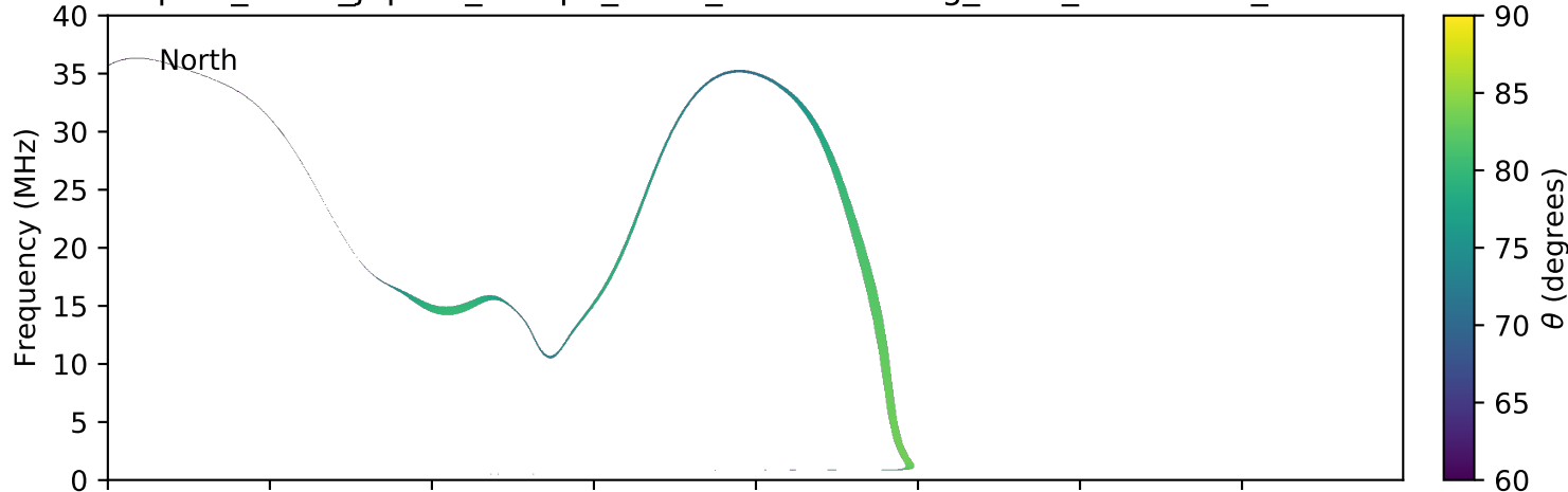
expres_earth_jupiter_europa_isaac_lossc-wid1deg_3kev_20160612_v01.cdf
