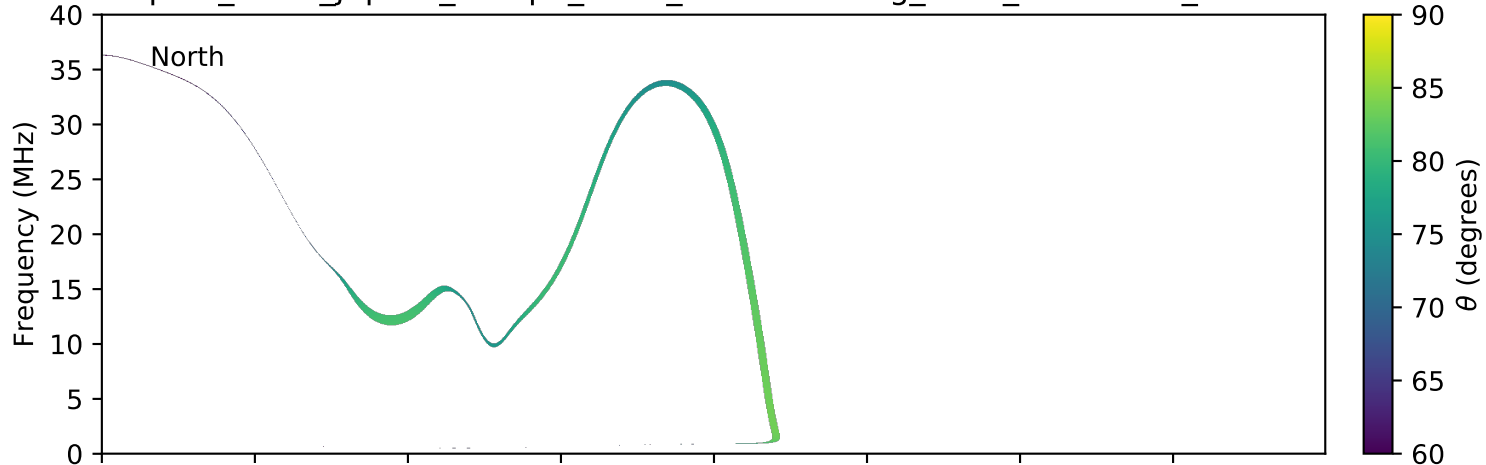
expres_earth_jupiter_europa_isaac_lossc-wid1deg_3kev_20160605_v01.cdf
