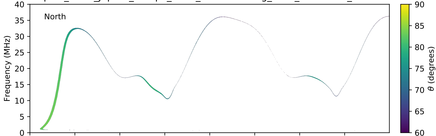
expres_earth_jupiter_europa_isaac_lossc-wid1deg_3kev_20160604_v01.cdf
