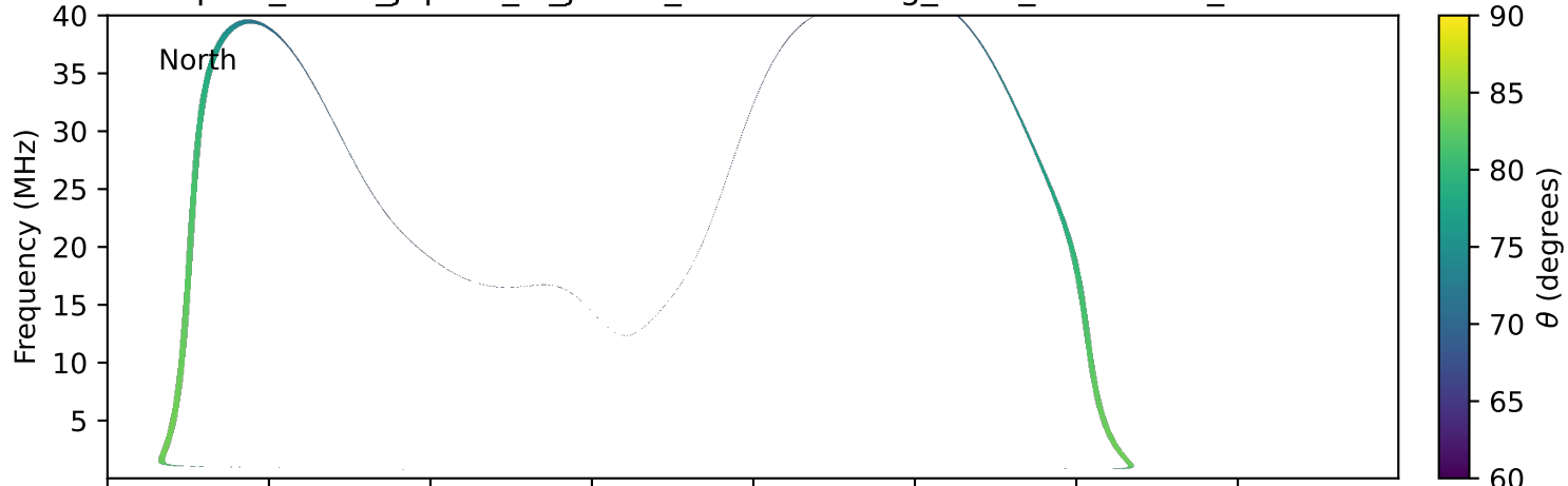
expres_earth_jupiter_io_jrm33_lossc-wid1deg_3kev_20160528_v11.cdf
