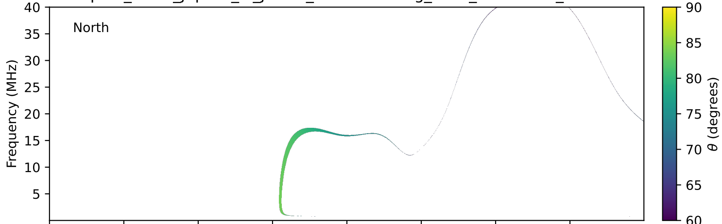
expres_earth_jupiter_io_jrm33_lossc-wid1deg_3kev_20160517_v11.cdf
