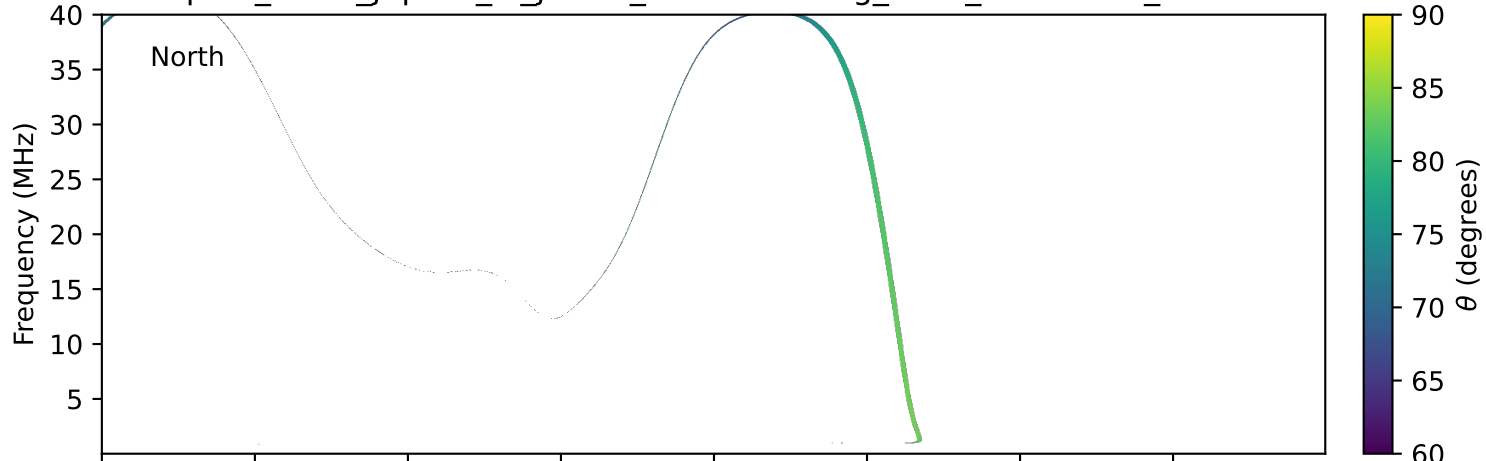
expres_earth_jupiter_io_jrm33_lossc-wid1deg_3kev_20160514_v11.cdf
