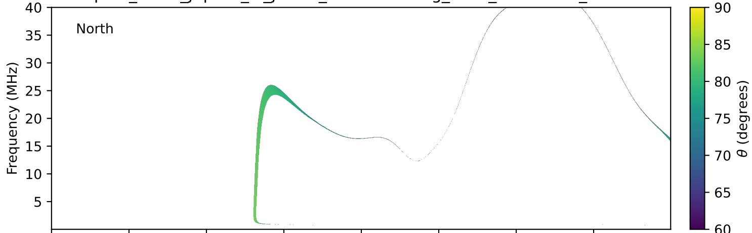
expres_earth_jupiter_io_jrm33_lossc-wid1deg_3kev_20160510_v11.cdf
