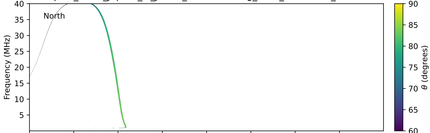
expres_earth_jupiter_io_jrm33_lossc-wid1deg_3kev_20160502_v11.cdf
